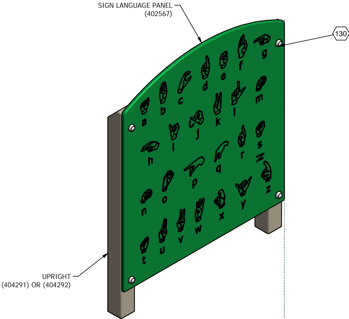
FINISHED ASSEMBLY
