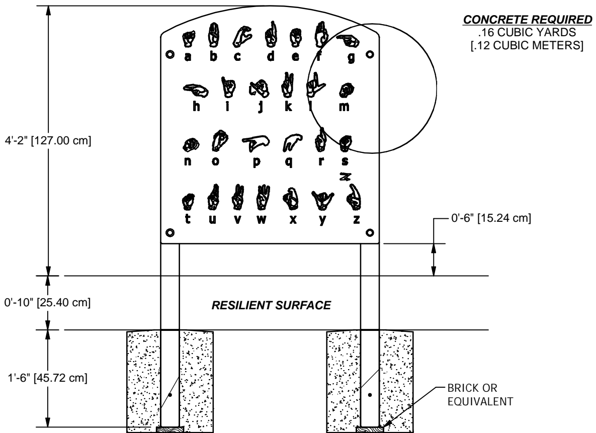
ELEVATION VIEW
