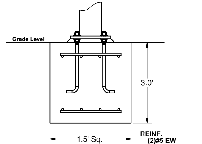
FOOTING DETAIL
