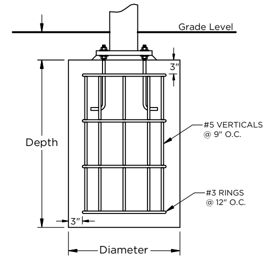
Typical Pier Footing
