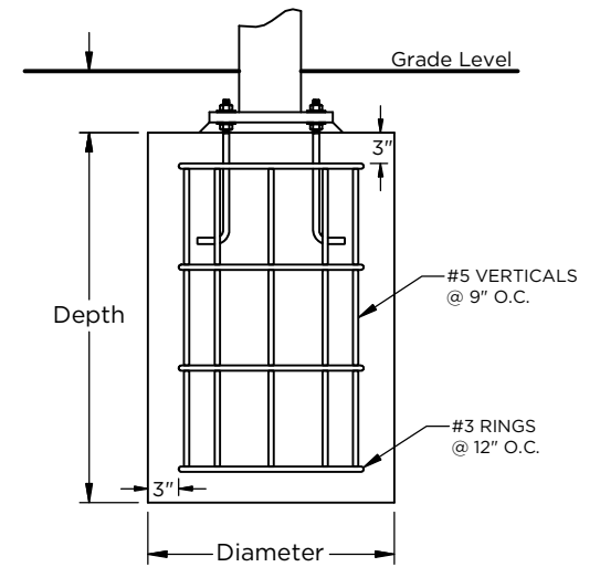
Typical Pier Footing
