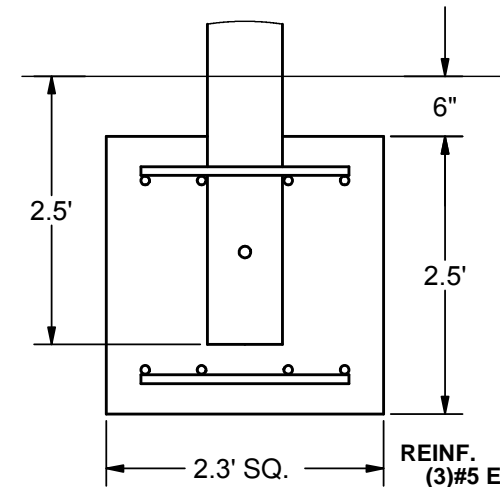
FOOTING DETAIL
