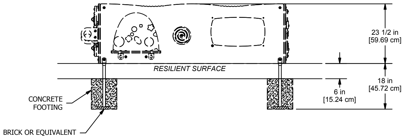
ELEVATION VIEW
